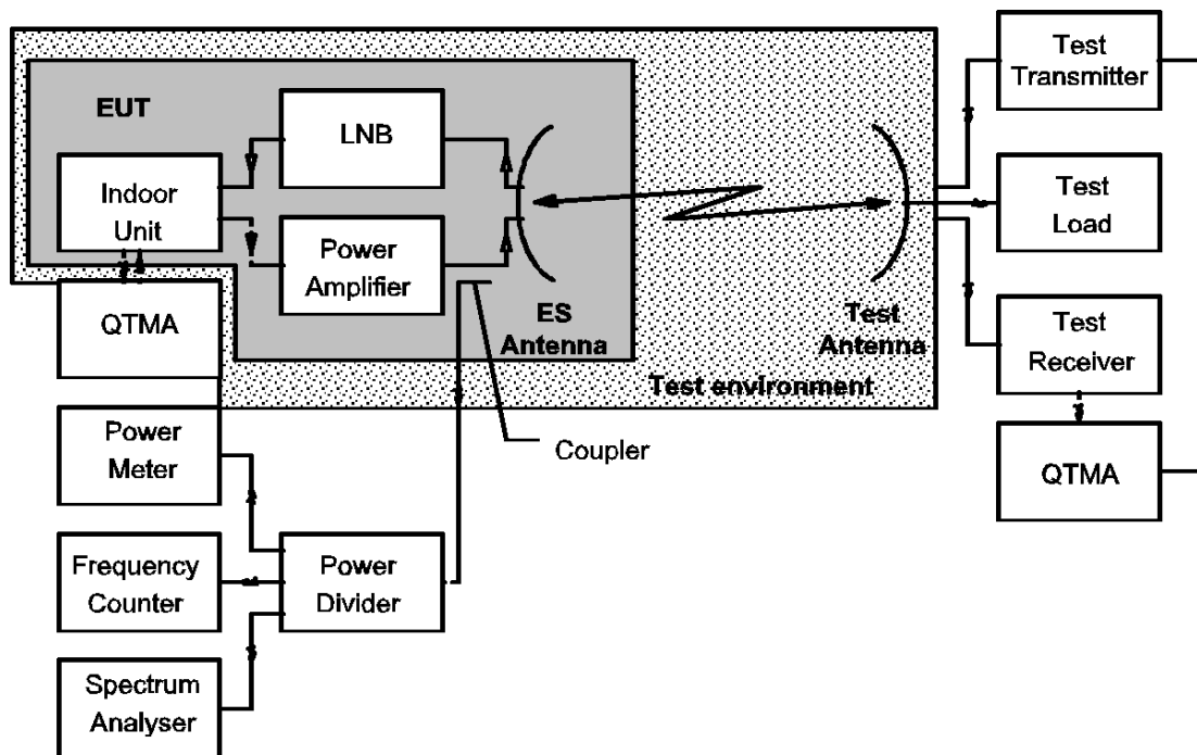
Figure 1: Test configuration
